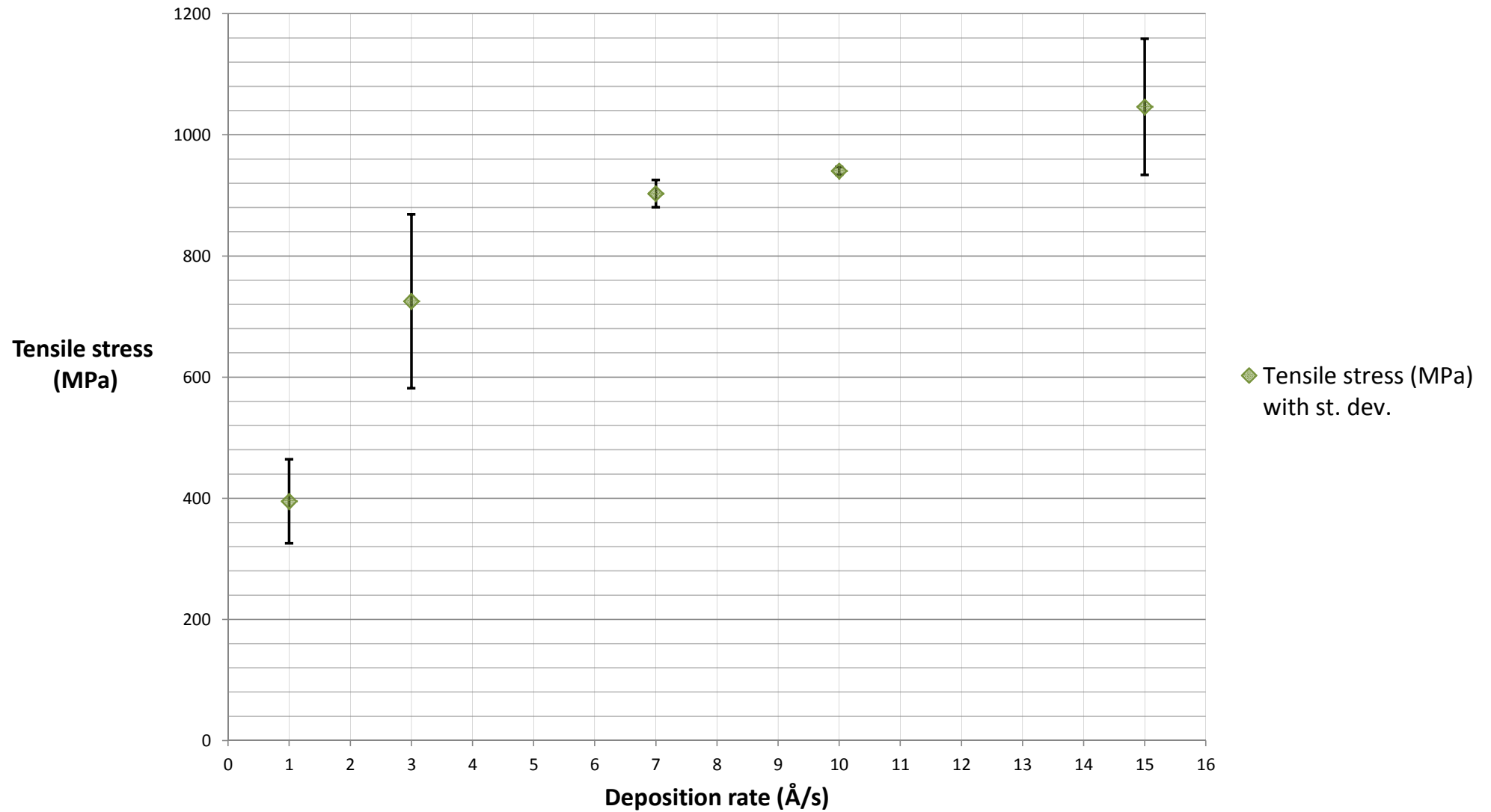
Tensile stress (MPa) as a function of deposition rate
