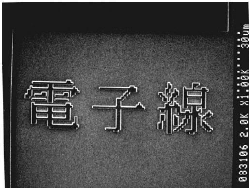
With ESPACER Charging Phenomenon on the EB Lithography Process
